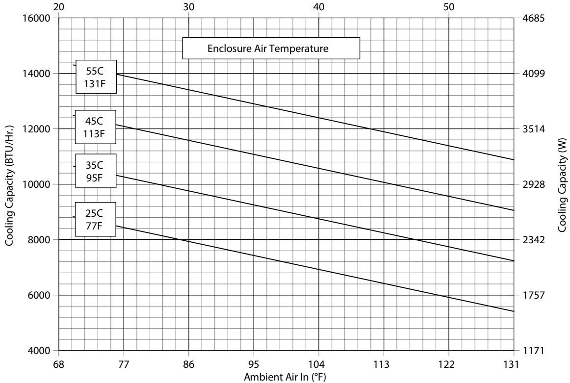
N43-1246-GXXX Capacity Curves at 60 Hz Ambient Air In (°C)
