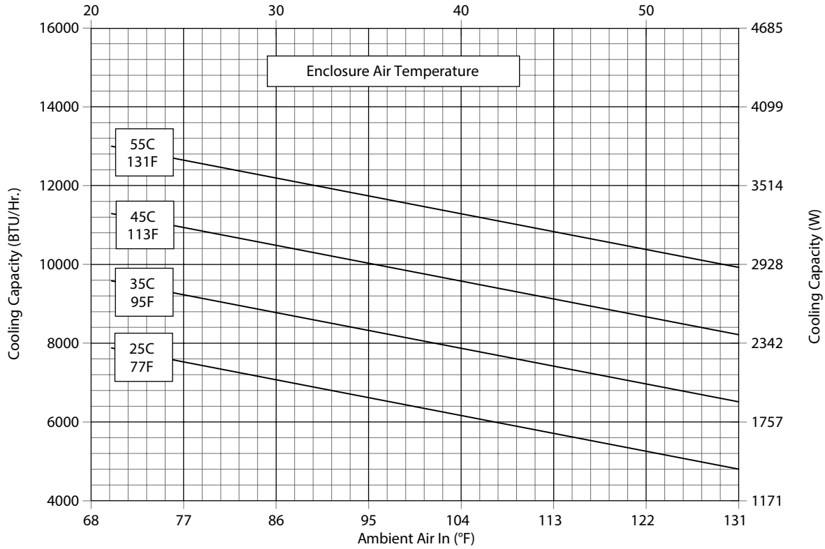
N43-1246-GXXX Capacity Curves at 50 Hz Ambient Air In (°C)
